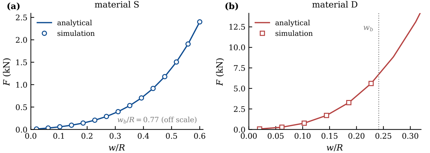
FIG. 4. Restoring force versus hub deflection for a star net with N = 8 radials, R = 1 m, \epsilon_p = 0.1 \epsilon_b : (a) material S, (b) material D. Lines: Eq. (12); markers: quasi-static simulation. Dotted line: failure at w_b (Table III); for S, w_b/R = 0.77 lies beyond the plotted range.
